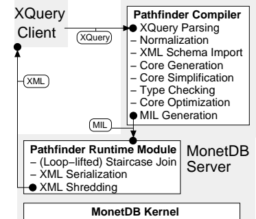
Figure 1: MonetDB/XQuery Architecture
