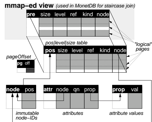
Figure 6: New Updateable Schema
